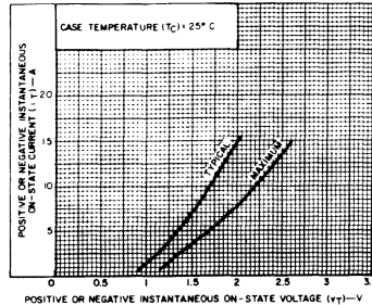
Fig. 8—On-state current vs. on-state voltage for all standard series.
