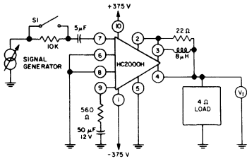
Fig.12 – Circuit for measurement of common-mode input impedance.
