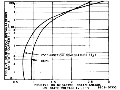
Fig. 9 - On-state current as a function of on-state voltage for SC151 series.
