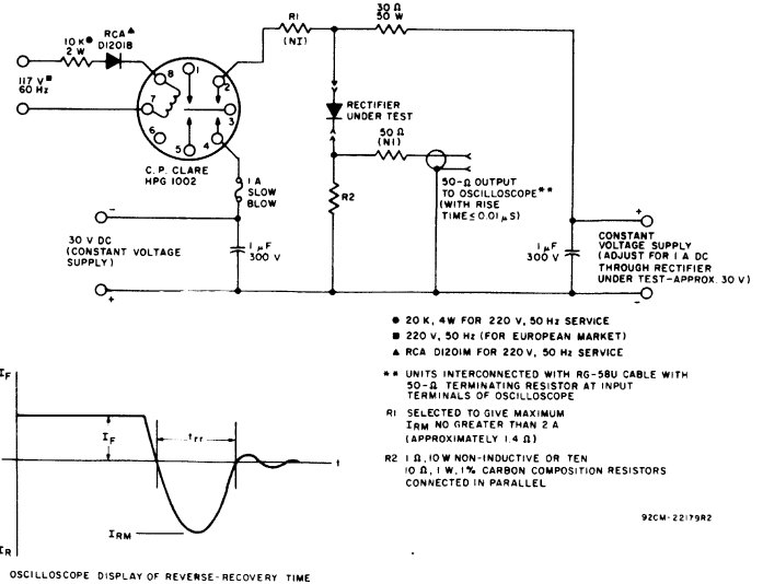
Fig.46 - Test circuit (pulsed dc) for measurement of reverse-recovery time.
