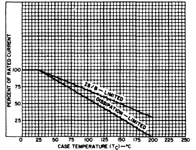
Fig. 2 - Dissipation and I B /θ derating curves for both types.
