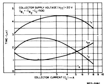
Fig. 10 - Typical saturated switching-time characteristics for all types.
