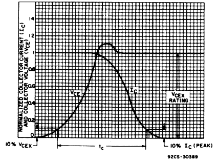
Fig. 16 - Oscilloscope display for normalized measurement of clamped inductive saturation switching time ( t_c ).
