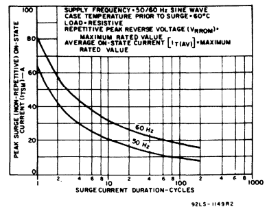
Fig. 2 — Peak surge on-state current vs. surge current duration for S3705M and S3706E.
