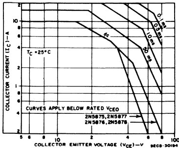
Fig. 1 - Collector-emitter voltage (V CE )-I C .
