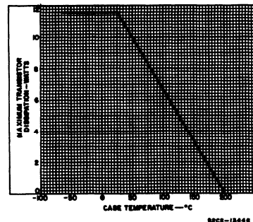
Fig. 2 - Dissipation derating chart.
