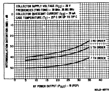
Fig. 1 - Typical intermodulation distortion as a function of rf power output.
