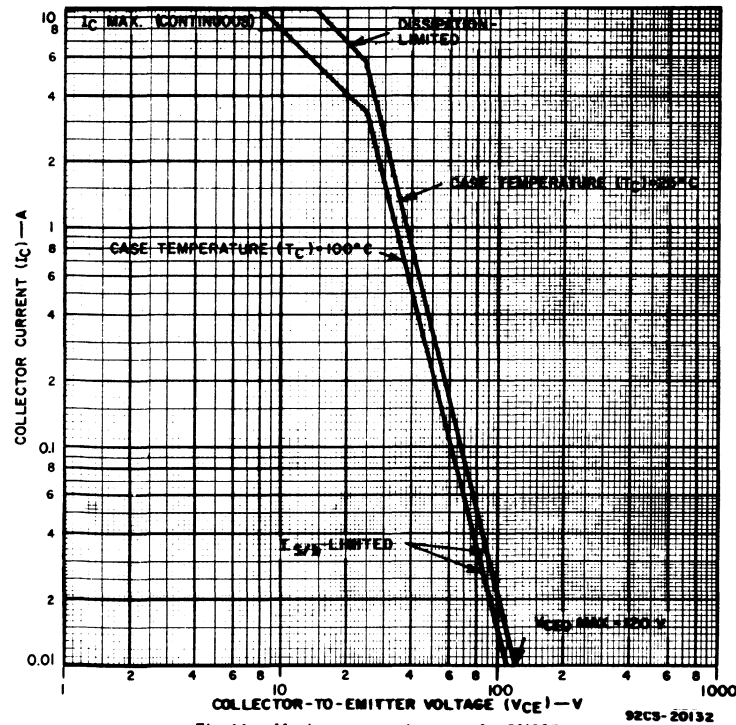
Fig. 11 - Maximum operating areas for 2N6354.
