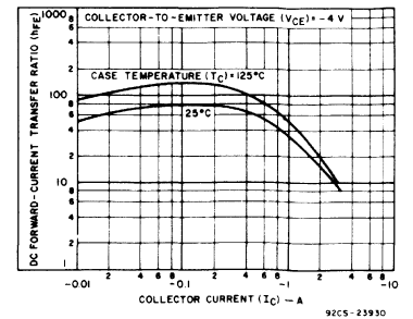
Fig. 13 - Typical dc beta characteristics for 41501.
