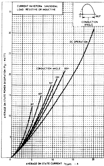
Fig. 1 - Power dissipation vs. on-state current.
