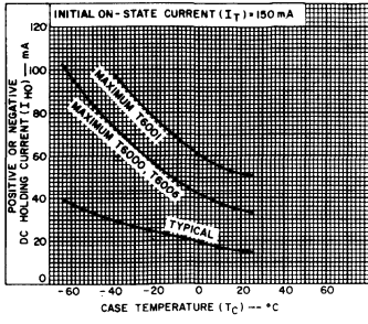
Fig. 7 — DC holding current vs case temperature.
