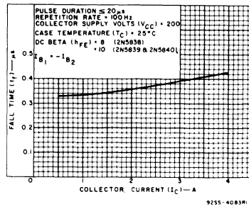
Fig. 12 - Typical fall-time characteristic for all types.
