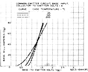
Fig. 4 - Typical input characteristics for 2N1483-2N1486, and 40368.
