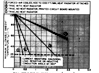
Fig. 3 - Maximum allowable ambient temperature vs. on-state current.
