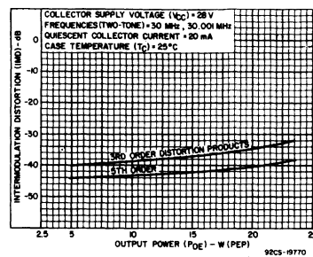
Fig. 1 - Typical intermodulation distortion as a function of output power.
