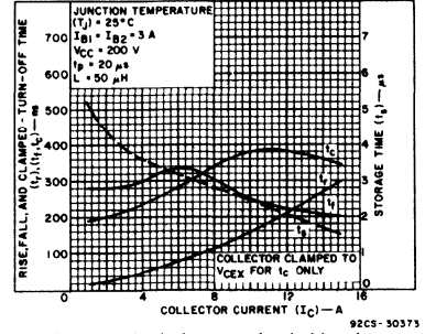
Fig. 10 - Typical saturated-switching-time characteristics at T_J = 25^\circ\text{C} as a function of collector current for all types.
