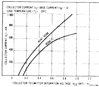
Fig. 21—Typical saturation characteristics for 40347, 40348 and 40349.
