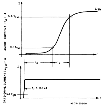
Fig.31 - Relationship between anode current (on-state), gate drive current, and time showing reference points for definition of gate controlled turn-on time ( t_{gt} ) for gate-turn-off SCR's.
