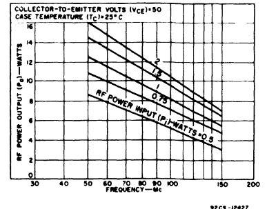
Fig. 3 - Typical operation characteristics.
