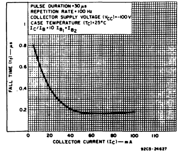
Fig. 6 - Typical fall-time characteristic for all types.
