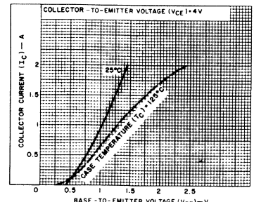
Fig. 13 - Typical transfer characteristics for RCA6263.
