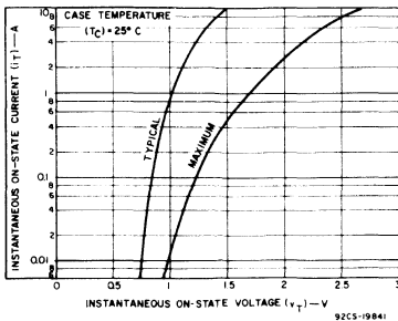
Fig. 8 - Instantaneous on-state current as a function of on-state voltage for all series.
