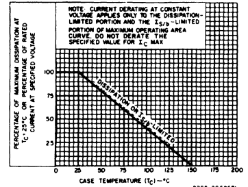
Fig. 2 - Derating curve.
