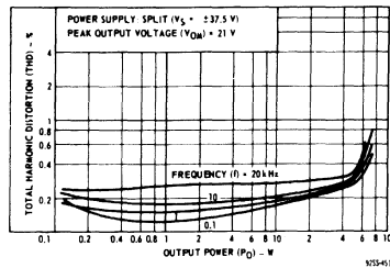
Fig. 10 - Total harmonic distortion with split power supply for HC2000H.
