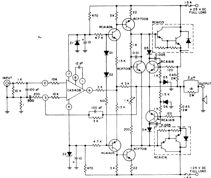
(a) Amplifier with ac coupling
