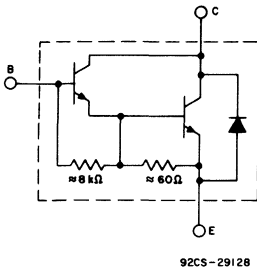
Fig. 1 - Schematic diagram for 2N6282, 2N6283, and 2N6284.
