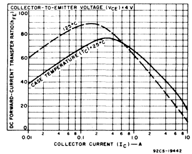
Fig. 6 - Typical dc-beta characteristics for 2N6254.
