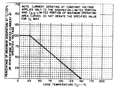
Fig. 2—Dissipation derating curve at case temperature for all types.
