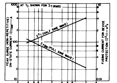
Fig. 6 - Peak surge on-state current and fusing current vs. time.
