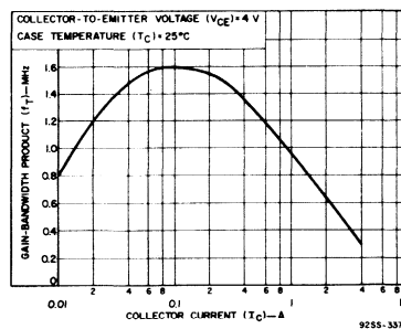
Fig. 2 — Typical gain-bandwidth product for all types.
