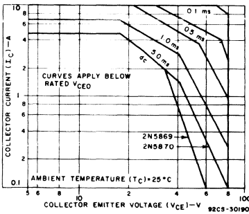
Fig. 1 - Maximum operating areas.
