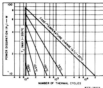
Fig. 2 - Thermal-cycling rating chart for all types.
