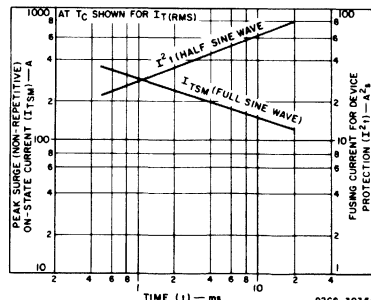
Fig. 7 - Peak surge on-state current and fusing current as a function of time.
