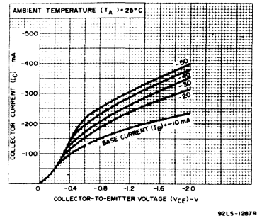
Fig.11—Typical small-signal output characteristics for 2N4037, 2N4314, 40391, and 40394.
