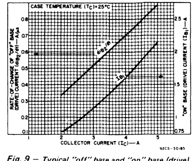
Fig. 9 — Typical "off" base and "on" base (drive) current as a function of collector current. See also "Guide for Optimizing 'ON' and 'OFF' Base (Drive) Current Conditions'".
