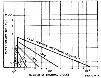
Fig. 4 - Thermal-cycling rating chart for RCS31-series
