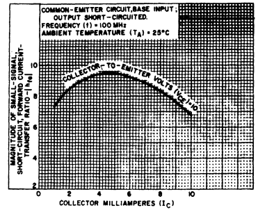
Fig. 1 - Typical small-signal beta characteristics for 2N5180.
