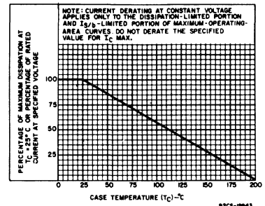
Fig. 3 - Derating curve for both types.
