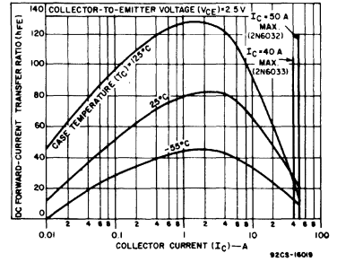
Fig. 2 - Typical de-beta characteristics for both types.
