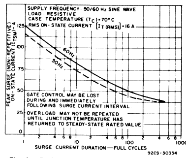
Fig. 4 - Peak surge on-state current as a function of surge current duration for TIC246 series.
