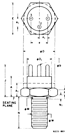
TO-212MA/TO-60
