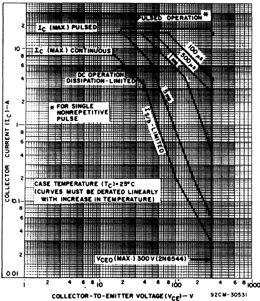
Fig. 15 - Maximum operating areas for type 2N6544 ( T_C = 25^\circ\text{C} ).
