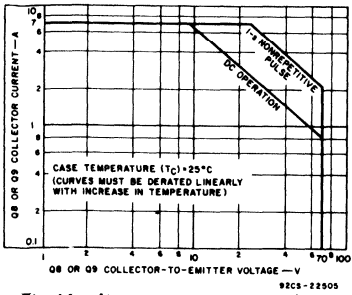
Fig. 14 - Maximum operating area for HC2500.
