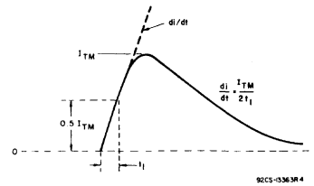
Fig. 25 - Rate of change of on-state current with time (defining di/dt) for an SCR.
