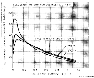
Fig. 3— Typical dc beta characteristics for 2N1479-2N1482.
