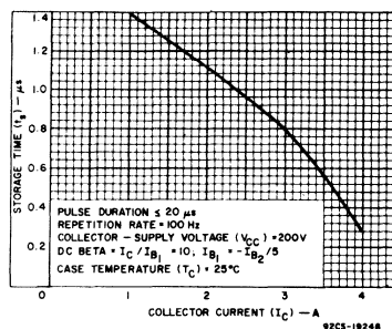
Fig. 9—Typical storage time vs. collector current.
