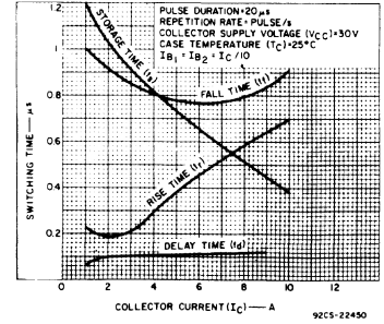
Fig. 9 - Typical saturated switching characteristics for 2N6486, 2N6487, and 2N6488.
