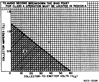
Fig. 1 - Region of safe operation for class A service. For class A operation must be located in region A.
