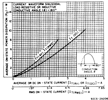
Fig. 4 — Power dissipation as a function of average, dc, or rms on-state current for C107 series.
