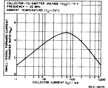
Fig. 5—Typical small-signal beta characteristics for all types.
