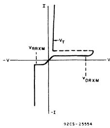
Fig. 22 - Anode-cathode voltage-current characteristic for a gate-turn-off SCR (GTO).
