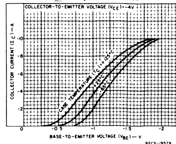
Fig. 4 - Typical transfer characteristics for 2N6246, 2N6247, 2N6248, and 2N6469.
