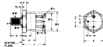
TO-211MB/TO-63
