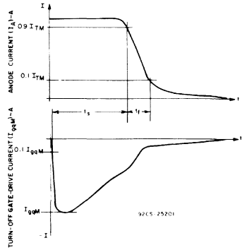
Fig. 38 — Relationship between anode current (on-state), turn-off gate-drive current, and time showing reference points for definition of gate-controlled turn-off time ( t_{qq} ).
