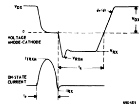
Fig.36 - Relationship between off-state voltage, reverse voltage, on-state current, and reverse current showing reference points for specification of turn-off time ( t_q ) for an inverter SCR (half-sine-wave pulse).
