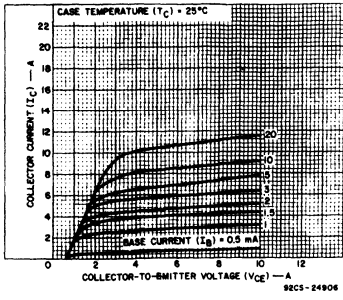
Fig. 10 - Typical output characteristics for all types.
