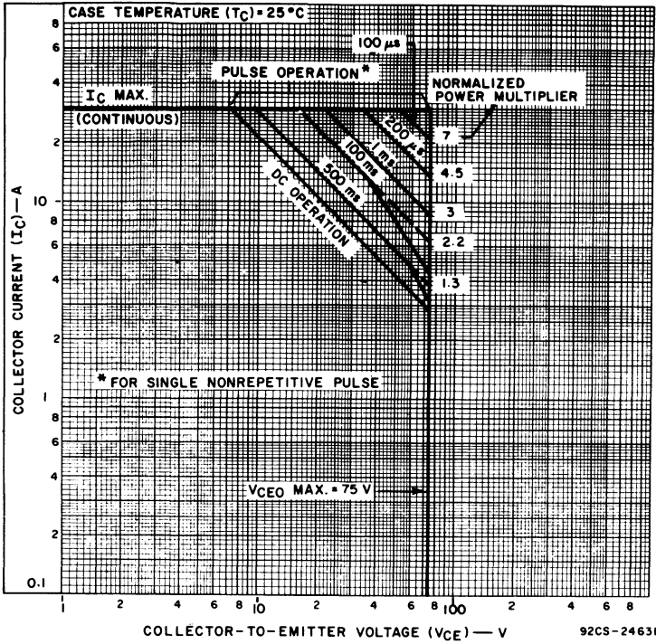
Fig. 3 - Maximum operating areas.
