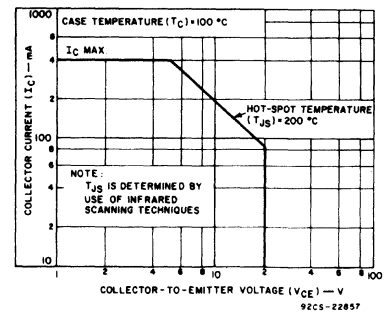
Fig. 2 - Safe area for dc operation.
