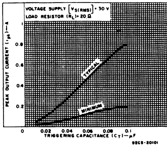
Fig. 1 — Peak output current vs. triggering capacitance.
