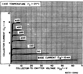
Fig. 10 - Typical output characteristics for 2N6098, 2N6099, and RCA3055.
