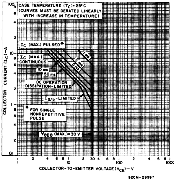
Fig. 2 - Maximum operating areas at T_C = 25^\circ\text{C} .
