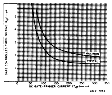
Fig. 12 — Turn-on time vs gate-trigger current.
