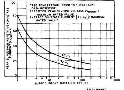
Fig. 5—Peak surge on-state current vs. surge-current duration.
