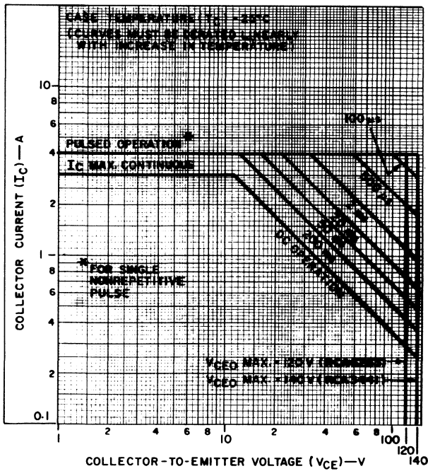
Fig. 11 - Maximum operating areas for RCA3441, RCA6263.
