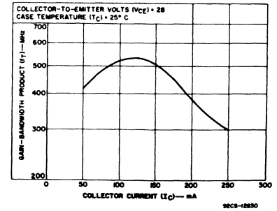
Fig. 2 - Gain-bandwidth product as a function of collector current.
