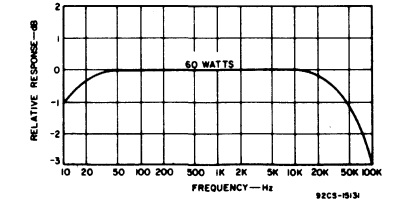
Fig. 7 - Typical response as a function of frequency at 60-W output for the 70-W amplifier.
