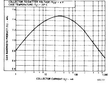
Fig. 15—Typical gain-bandwidth product for 2N5295 and 2N5296.
