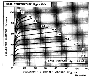
Fig. 7—Typical output characteristics for 2N3439, 2N3440, 2N4063, 2N4064 and 40390.
