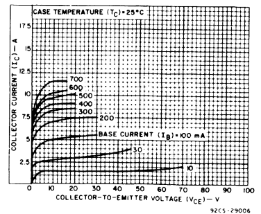
Fig. 8 — Typical output characteristics. ♦
