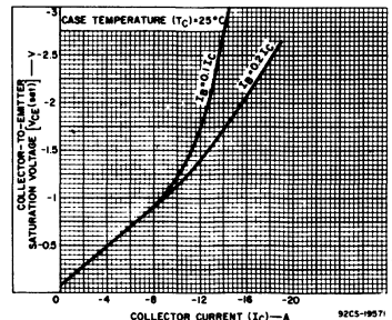
Fig. 2 - Typical collector-to-emitter saturation-voltage characteristics for 2N6246, 2N6247, 2N6248, and 2N6469.
