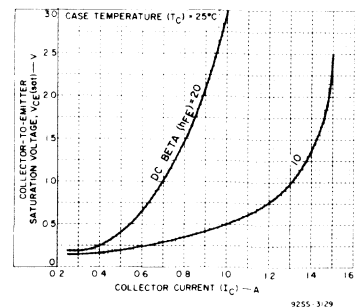
Fig. 3—Typical collector-to-emitter saturation voltage vs. current for 2N3584 and 2N3585.
