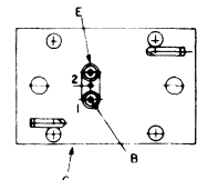
JEDEC TO-66 with Heat Radiator 40373, 40912, 40913
