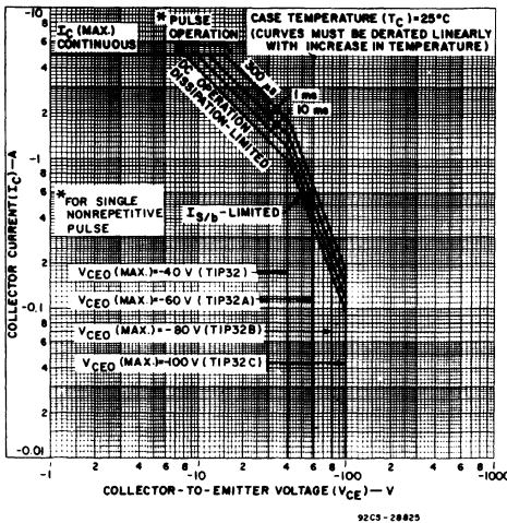
Fig. 1 - Maximum operating areas for TIP32-series.
