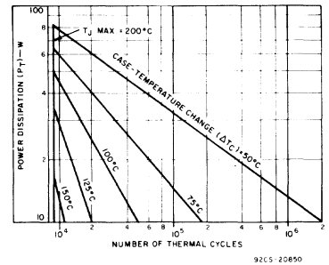
Fig. 2 — Thermal-cycling ratings for RCA1B01.
