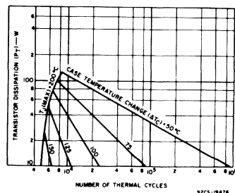
Fig. 1 - Thermal-cycle rating chart for all types.
