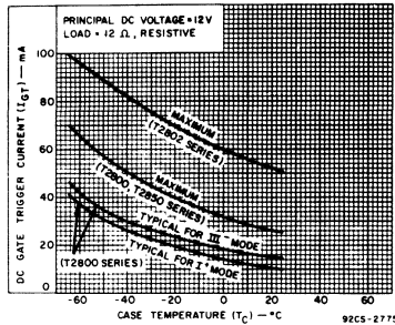
Fig. 12 - DC gate-trigger current (for I_{T1} and III^{-} triggering modes) vs. case temperature for T2800, T2802, T2850 series.
