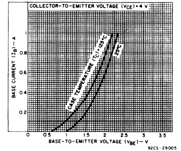
Fig. 7 — Typical input characteristics. ♦
