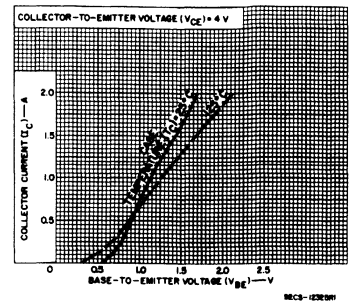
Fig. 14 - Typical transfer characteristics for 2N3054, 2N6260, 40250, 40250V1, 40372 and 40910.
