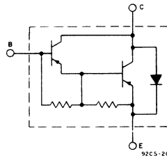
Fig. 2 - Schematic diagram for RCA1C16.
