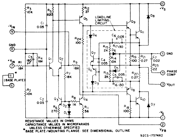
Schematic diagram of type HC2000H operational amplifier.
