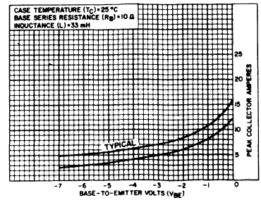
Fig. 8 - Reverse-bias second-breakdown characteristics for both types.
