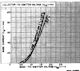
Fig. 9 - Typical input characteristics for 2N3054, 2N6260, 40250, 40250V1, 40372, and 40910.
