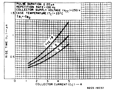
Fig. 9 - Typical rise-time characteristic for all types.
