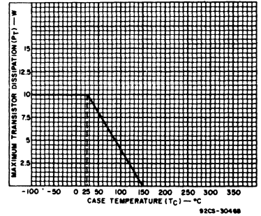
Fig. 1 - Derating curve.
