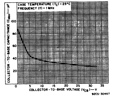
Fig. 6 — Typical collector-to-base capacitance as a function of collector-to-base voltage.
