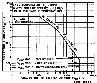
Fig. 2 - Maximum operating areas for all types, at T_C = 100^\circ C .
