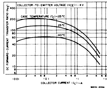
Fig. 3 - Typical dc beta characteristics for BD242-series types.
