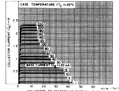
Fig. 6 - Typical output characteristics for 2N1701.
