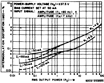
Fig. 20 - Typical intermodulation distortion vs. rms output power for HC2500.
