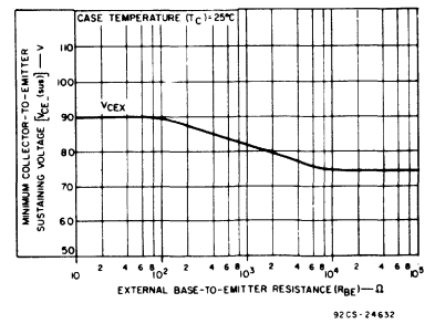
Fig. 8 - Sustaining voltage vs. base-to-emitter resistance.
