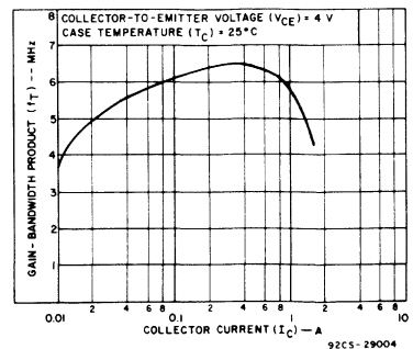
Fig. 8 - Typical gain-bandwidth product for both types.
