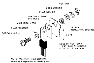
TO-202AB
