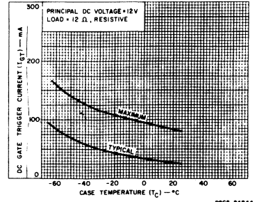
Fig. 10 - DC gate-trigger current (for I + and III - triggering modes) as a function of case temperature.
