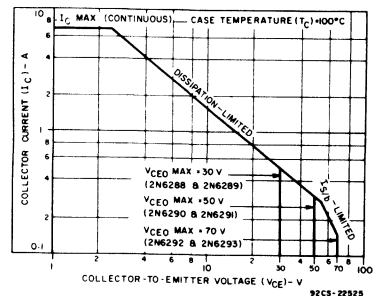
Fig. 19 - Maximum operating areas for 2N6288-2N6293.
