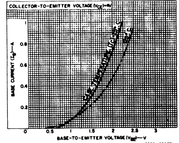
Fig. 14 - Typical input characteristics for 2N3055 (Hometaxial), 2N6371 and 40251.
