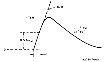
Fig. 24 - Rate of change of on-state current with time (defining di/dt) for a triac.
