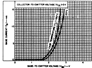
Fig. 6 - Typical input characteristics for all types.
