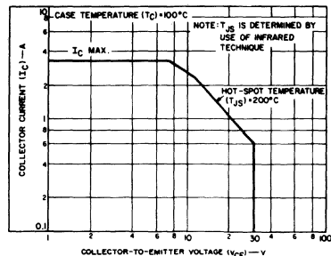
Fig. 2 - Maximum operating area for forward-bias operation.
