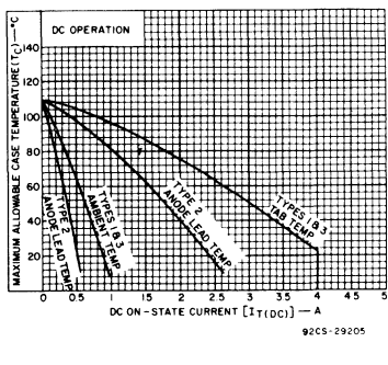
Fig. 3 — Maximum allowable case temperature as a function of dc on-state current for C106 series.
