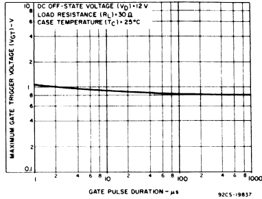
Fig. 12 - Maximum gate trigger voltage as a function of gate pulse duration for types in the S106 series.
