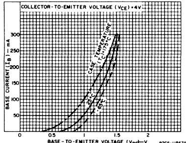
Fig. 5 - Typical input characteristics for 2N1702.
