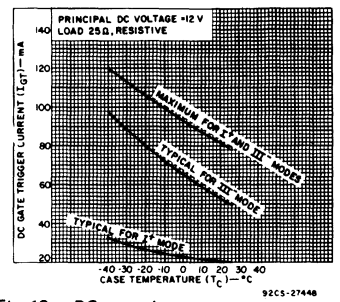
Fig. 18 - DC gate-trigger current vs. case temperature ( I^+ & III^- modes) for 2N5806-2N5809.
