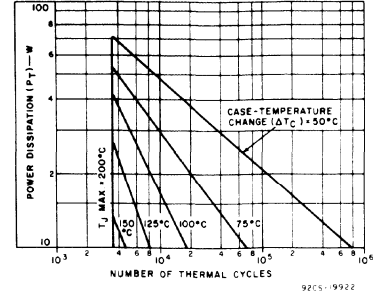
Fig. 3 - Thermal-cycling rating chart for 2N6055-2N6056, 2N6383-2N6385.
