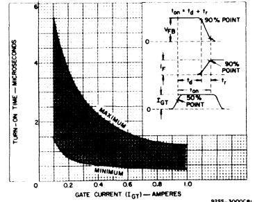
Fig. 8 - Turn-on time characteristics.
