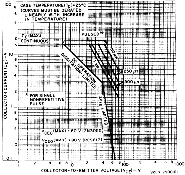
Fig. 9 — Maximum operating areas for 2N3055 and RCS617.
