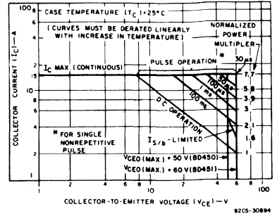
Fig. 4 - Maximum operating areas.
