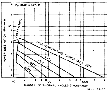
Fig. 1 - Thermal-cycling rating chart for all types.
