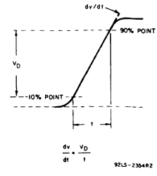
Fig. 28 - Rate of rise of off-state voltage with time (defining dv/dt) for an inverter SCR.
