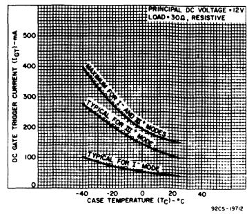
Fig. 8 - DC gate-trigger current vs. case temperature ( I^- and III^+ modes) for T8411 and T8421 series.
