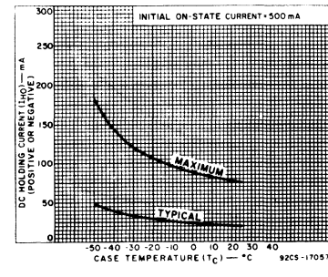
Fig. 5—DC holding current vs. case temperature.
