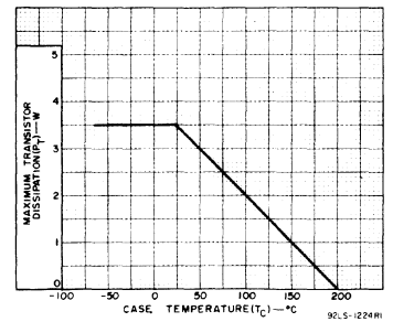
Fig. 1 - Derating curve.
