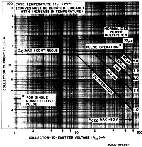
Fig. 7 - Maximum operating areas for 2N6254.
