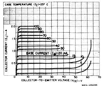
Fig. 7 – Typical output characteristics.
