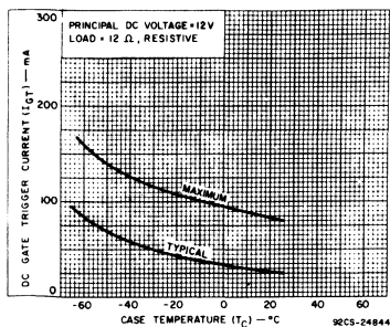
Fig. 14 - DC gate-trigger current (for I_{T1} and III^{-} triggering modes) vs. case temperature for T2801 series.
