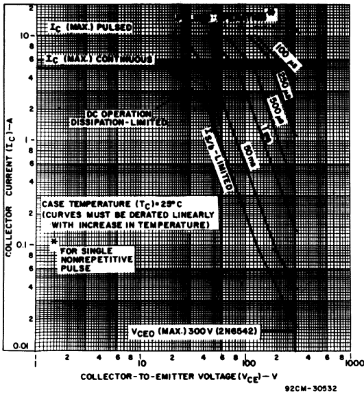
Fig. 1 - Maximum operating areas for type 2N6542 (T C = 25°C).
