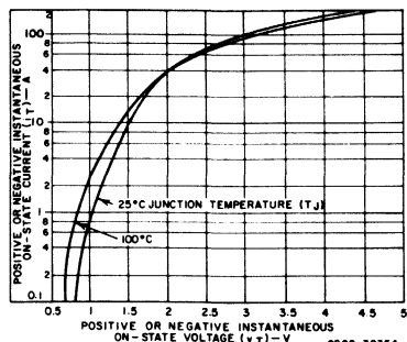
Fig. 8 - On-state current as a function of on-state voltage for SC149 series.
