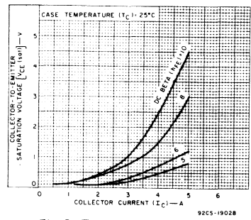
Fig. 6 - Typical saturation voltage characteristics for all types.
