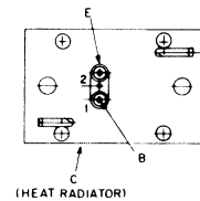
JEDEC TO-66 with Heat Radiator 40250V1, 40372, 40910, 40911
