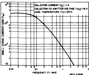
Fig. 7 - Typical small-signal current gain for all types.
