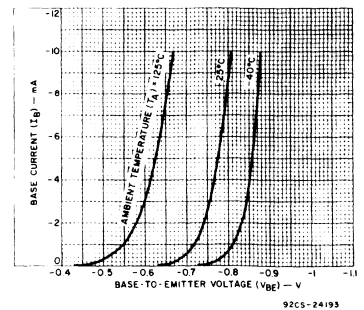
Fig. 11 - Typical input characteristics for RCP700, RCP702, RCP704, RCP706-series types.
