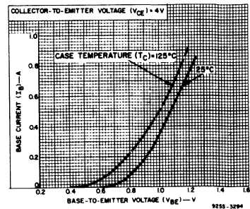
Fig. 7 - Typical input characteristics.
