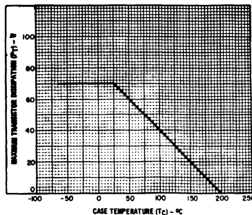
Fig. 2 - Dissipation derating chart.
