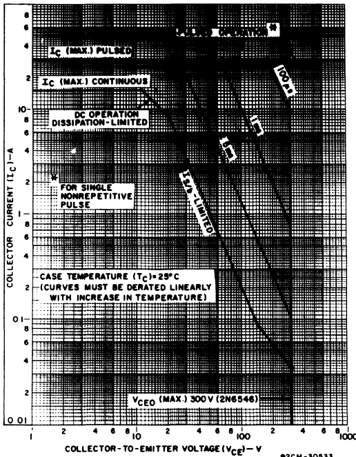
Fig. 14 - Maximum operating areas for type 2N6546 ( T_C = 25^\circ\text{C} ).
