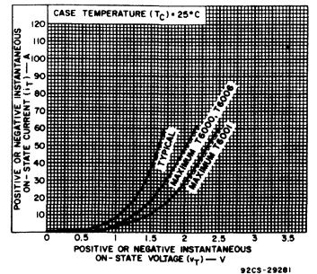
Fig. 6 - On-state current vs on-state voltage.
