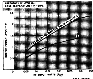
Fig. 2 - Typical power output as a function of power input at 250 MHz.
