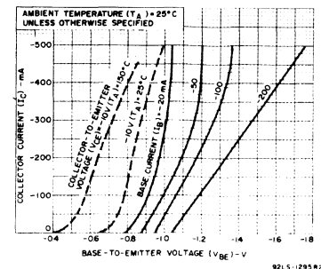
Fig. 7—Typical transfer characteristics for 2N4037 and 2N4314.
