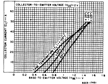
Fig. 3 - Typical transfer characteristics for both types.
