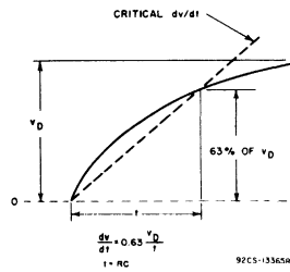
Fig. 27 - Rate of rise of off-state voltage with time (defining critical dv/dt) for general-purpose SCR's, gate-turn-off SCR's, and triacs.
