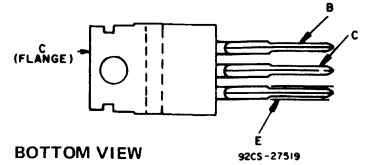
TO-220AB
