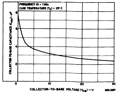
Fig. 5 - Typical variation of collector-to-base capacitance with collector-to-base voltage.
