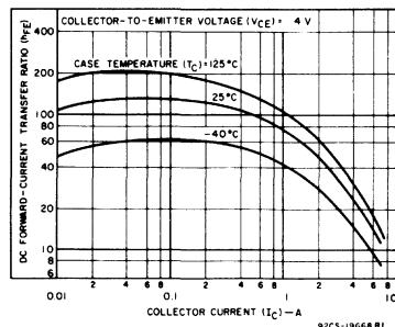
Fig. 2 - Typical dc beta characteristics for BD243-series types.
