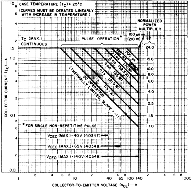
Fig. 9—Maximum operating areas for 40347, 40348, and 40349.
