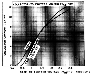
Fig. 7 – Typical transfer characteristics for MJ15001.
