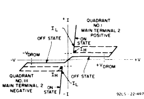
Fig. 20 - Principal voltage-current characteristic for a triac.
