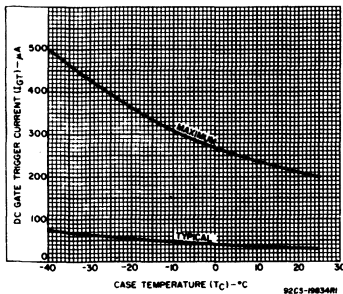
Fig. 10—DC gate-trigger current vs. case temperature for S2060 series.
