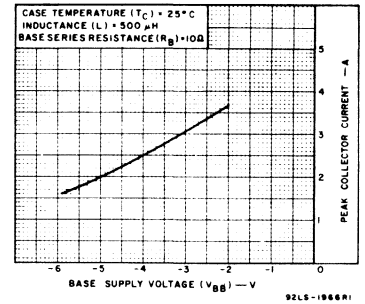
Fig. 9 - Typical reverse bias, second-breakdown characteristic for all types.
