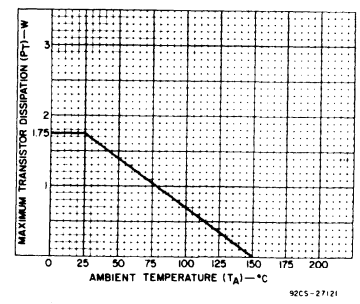
Fig. 3—Dissipation derating curve at ambient temperature for all types.
