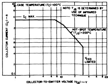
Fig. 3 - Safe operation with dc forward bias.
