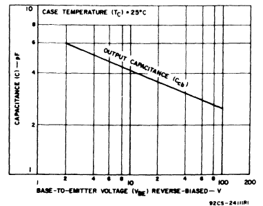
Fig. 8 - Typical junction capacitance vs. reverse-bias base-to-emitter voltage.
