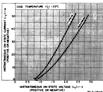
Fig. 8 — On-state current vs. on-state voltage for all 15-A triacs.
