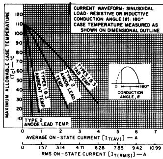
Fig. 8 - Maximum allowable case temperature as a function of average or rms on-state current for C108 series.
