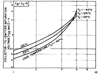
Fig. 5 - Typical collector-to-emitter saturation voltage as a function of collector current for all types.
