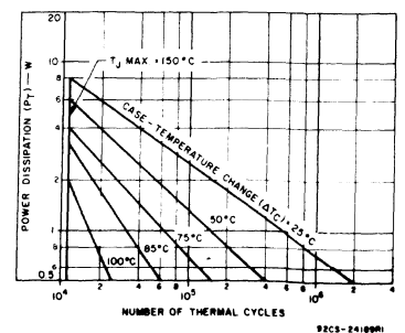
Fig. 4—Thermal-cycling rating chart for all types.
