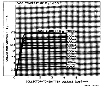
Fig. 11—Typical output characteristics for 2N3771.
