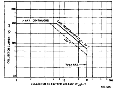
Fig. 1 - Safe area for dc operation.
