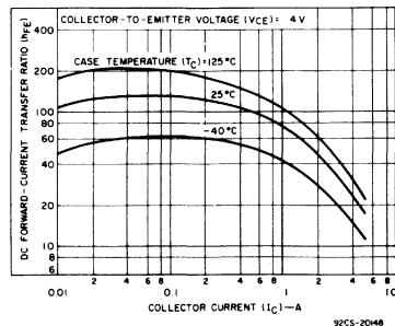
Fig. 2 - Typical dc beta characteristics for BD241-series types.
