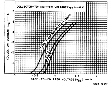
Fig. 7 - Typical transfer characteristics for 2N6475 and 2N6476.
