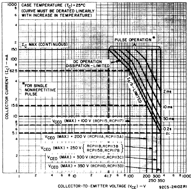
Fig. 7 - Maximum operating areas for all types.
