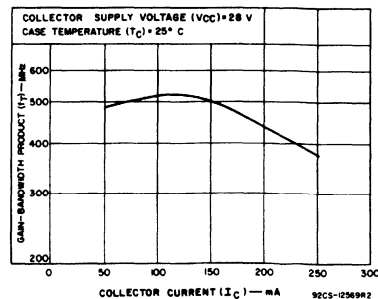
Fig. 3 - Typical gain-bandwidth product as a function of collector current.
