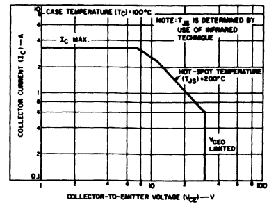
Fig. 3 - Safe operation area with dc forward bias.
