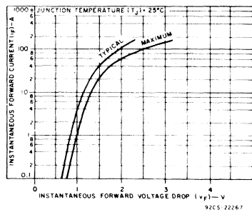
Fig. 6 - Forward current vs. forward voltage drop for D2412 series.
