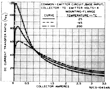
Fig. 1 - Typical dc beta characteristics for 2N1487-2N1490, and 40369.
