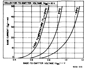
Fig. 13 — Typical input characteristics for BUX67-series types.
