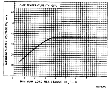
Fig. 7 - Maximum allowable supply voltage vs. load resistance for HC2000H.
