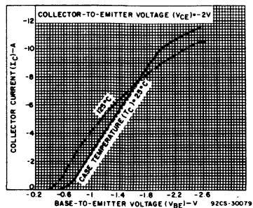
Fig. 8 – Typical transfer characteristics for MJ15002.
