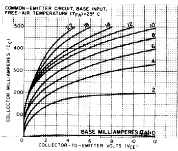
Fig. 20 - Typical high-current output characteristics for 2N699, 2N2270.
