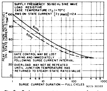
Fig. 3 - Peak surge on-state current as a function of surge current duration for TIC236 series.
