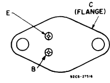
JEDEC TO-213MA
