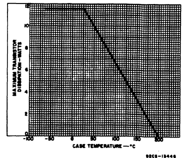
Fig. 5 - Dissipation derating curve.
