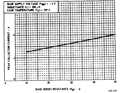
Fig. 9 - Typical reverse-bias, second-breakdown characteristic for both types.
