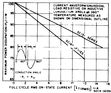
Fig. 4 - Maximum allowable case-temperature as a function of on-state current for both series.
