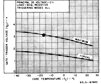
Fig. 15—Gate-trigger voltage vs. case temperature.
