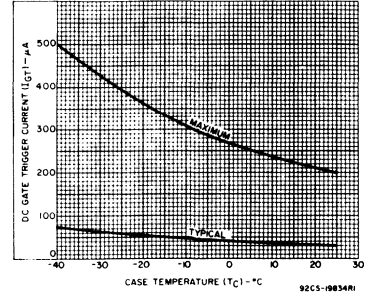
Fig. 13 - DC gate trigger current as a function of case temperature for S106 series.
