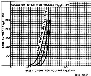
Fig. 12 - Typical input characteristics for 2N6467 and 2N6468.
