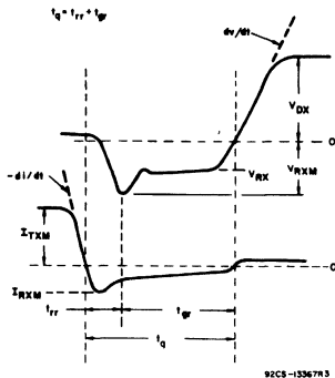
Fig.35 - Relationship between off-state voltage, reverse voltage, on-state current, and reverse current showing reference points defining turn-off time ( t_q ) for inverter SCR's (rectangular pulse).
