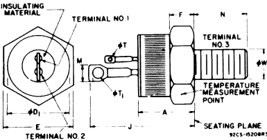
TO-208MA/TO-48
