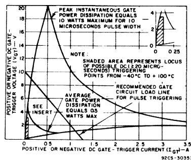
Fig. 7 - Gate pulse characteristics for all triggering modes.
