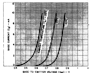
Fig. 16 - Typical input characteristics for RCP701, RCP703, RCP705, RCP707-series types.
