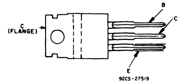
BOTTOM VIEW JEDEC TO-220AB
