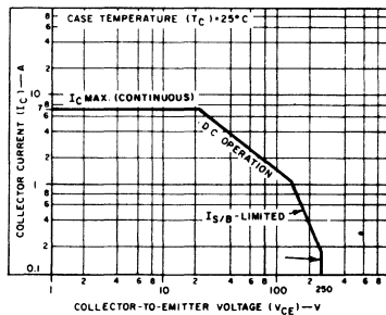
Fig. 4 - Maximum operating areas for RCA1B05.
