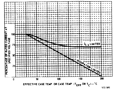
Note: Use ambient temperature for derating 40375. Fig. 2 - Dissipation derating for all types.
