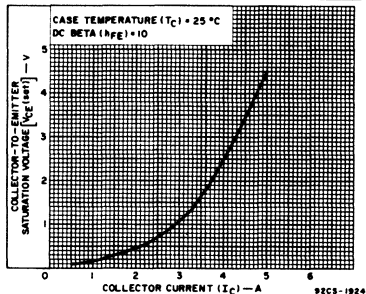
Fig. 6—Typical saturation voltage characteristic.
