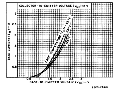
Fig. 6 - Typical input characteristic for 2N6496.
