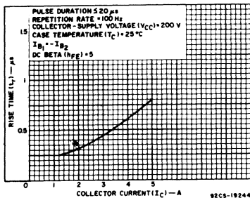
Fig. 8—Typical rise-time characteristic.
