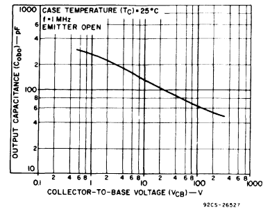
Fig. 6 - Typical output capacitance for all types.
