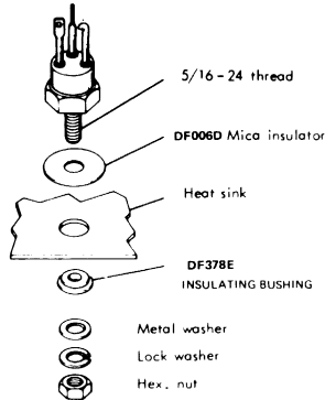
TO-211MB/TO-63
