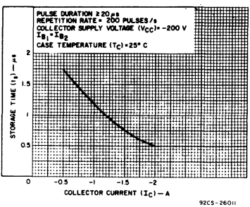
Fig. 18 — Typical storage-time characteristic for BUX66-series types.
