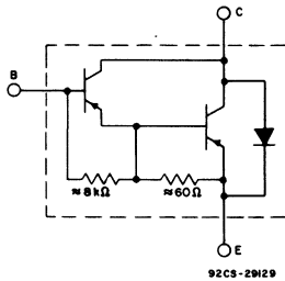
Fig. 2 - Schematic diagram for 2N6285, 2N6286, and 2N6287.
