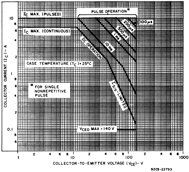
Fig. 4 - Maximum operating areas.
