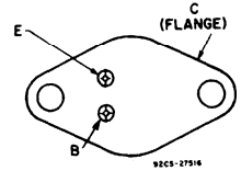
JEDEC TO-213MA RCA29-series
