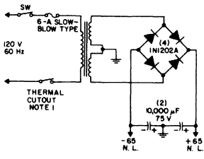
Fig. 10 - Power supply for 120-W audio amplifier circuit shown in Fig. 9.
