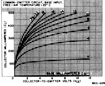
Fig. 23 - Typical high-current output characteristics for 2N1893.
