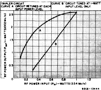
Fig. 3 - Power output as a function of power input.
