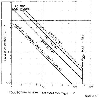
Fig. 10—Maximum operating areas for 40374.
