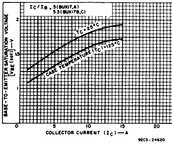
Fig. 7 - Typical base-to-emitter saturation-voltage characteristics for all types.
