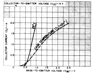
Fig. 12 - Typical transfer characteristics for RCA3441.
