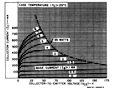
Fig. 10 — Typical output characteristics for BUX67-series types.
