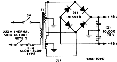
Fig. 5 - 70-watt amplifier circuit featuring quasi-complementary-symmetry output employing epitaxial-base construction output transistors: (a) basic amplifier circuit, (b) power-supply circuit.
