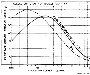
Fig. 12 - Typical dc beta characteristics for 2N4347.
