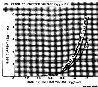
Fig. 5 — Typical input characteristics for 40407, 40408, and 40409.
