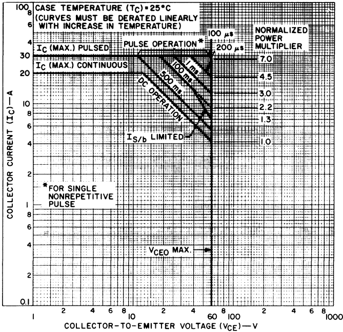
Fig. 8— Maximum operating areas for RCS258.
