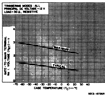
Fig. 11 — DC gate-trigger voltage vs. case temperature.
