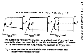
Fig. 9 - Oscilloscope display for measurement of sustaining voltages of p-n-p power transistors.
