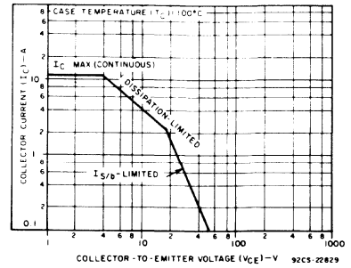
Fig. 6 - Maximum operating area for both types ( T_C = 100^\circ\text{C} ).
