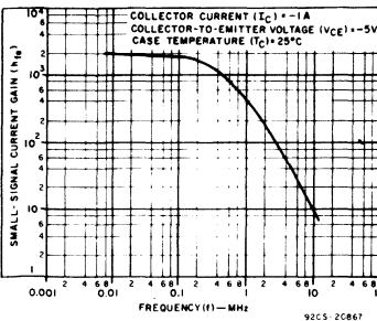
Fig. 15 - Typical small-signal gain for BDX34-series types.
