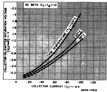
Fig. 5 - Typical collector-to-emitter saturation voltage.
