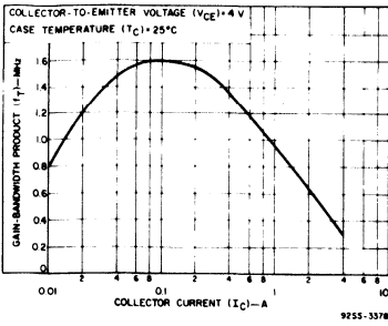
Fig. 10 — Typical gain-bandwidth product for all types.
