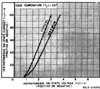
Fig. 7 — On-state current vs. on-state voltage for all 10-A triacs.
