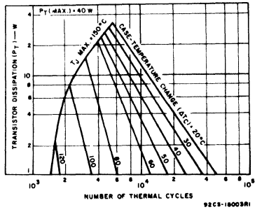
Fig. 1 - Thermal-cycling ratings for both types.
