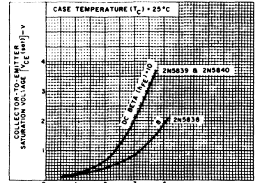
Fig. 3 - Typical saturation voltage characteristics for all types.
