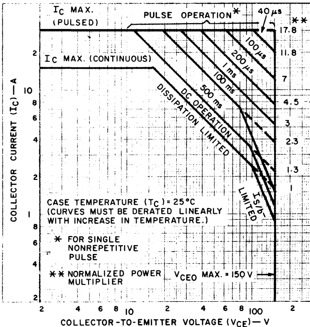
Fig. 14 - Maximum operating areas for 2N6259.
