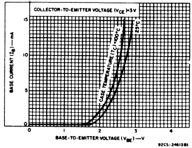
Fig. 8 — Typical input characteristics for both types.
