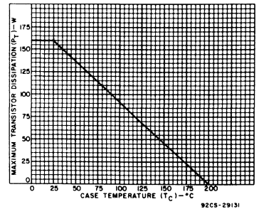
Fig. 3 - Power derating curve for all types.
