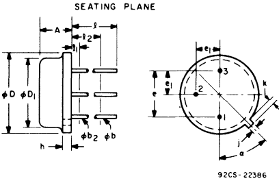
TO-206MB/TO-46
