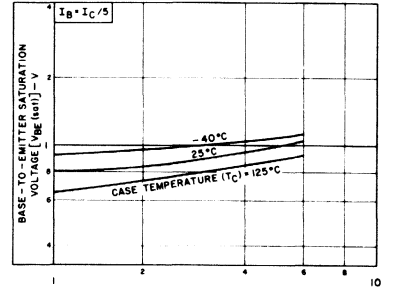
Fig. 6 - Typical base-to-emitter saturation voltage as a function of collector current for all types.
