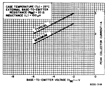
Fig. 16 — Reverse-bias second-breakdown characteristics for BUX67-series types.
