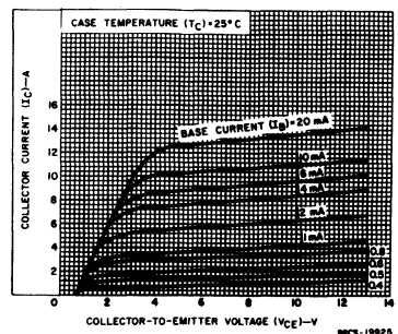
Fig. 5 - Typical output characteristics for 2N6386, 2N6387, and 2N6388.
