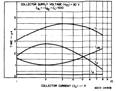
Fig. 12 - Typical saturated switching characteristics for all types.
