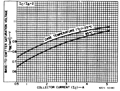
Fig. 4 - Typical base-to-emitter saturation voltage as a function of collector current.
