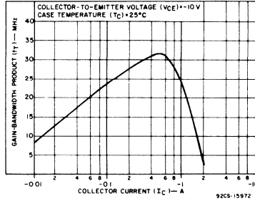
Fig. 5 - Typical gain-bandwidth product for all types.
