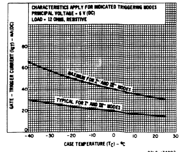
Fig. 6—DC gate-trigger current characteristics for I + and I III- modes.
