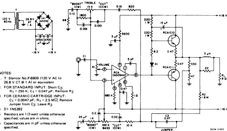
Fig. 5 - 12-watt amplifier circuit featuring an integrated-circuit driver and a true-complementary-symmetry output stage.
