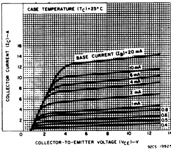
Fig. 9 – Typical output characteristic for all types.
