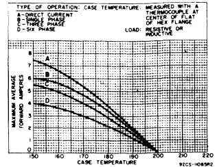
Fig. 1 -- Maximum average forward current vs. case temperature for 1N1341B, 1N1342B, 1N1344B-1N1348B.
