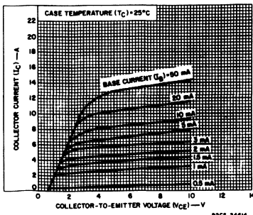
Fig. 9 — Typical output characteristics for both types.
