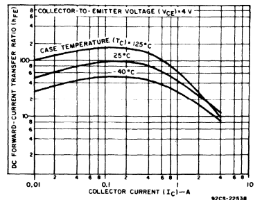
Fig. 6 - Typical dc beta characteristics for TIP31C, RCA31C and RCS31C.
