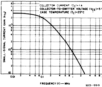
Fig. 12 - Typical small-signal gain for BDX33-series types.
