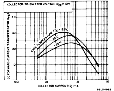
Fig. 2 - Typical dc beta vs. collector current for all types.
