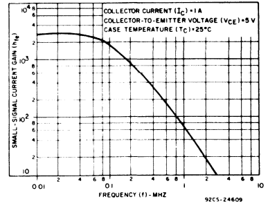
Fig. 6 — Typical small-signal gain for both types.
