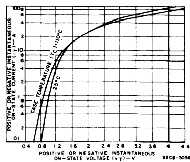
Fig. 8 - On-state current as a function of on-state voltage.
