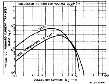
Fig. 4 - Typical dc-beta characteristics for BDX33-series types.
