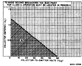
Fig. 1 - Region of safe operation (without second breakdown) in class A service for type 2N2876.
