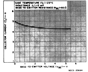
Fig. 6 – Minimum values of reverse-bias second-breakdown characteristic ( E_{S/b} ) b for all types.
