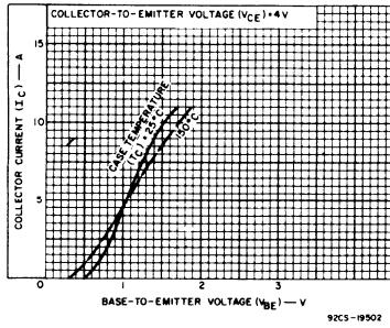
Fig. 10—Typical transfer characteristics for 2N3772, 2N6257 and RCS258.
