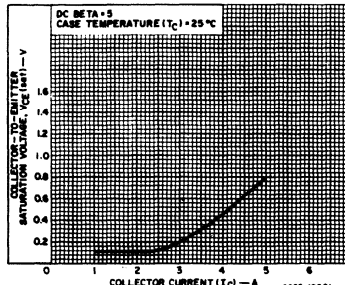
Fig. 6—Saturation voltage vs. collector current.
