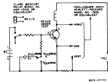
Fig. 8 - Basic circuit configuration used to measure sustaining voltages V_{CE0}(sus) , V_{CE(sus)} , and V_{CEV}(sus) for p-n-p power transistors.
