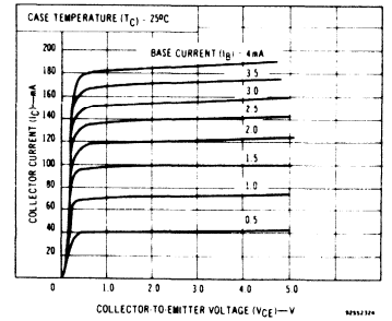
Fig. 13—Typical output characteristics for 40349.
