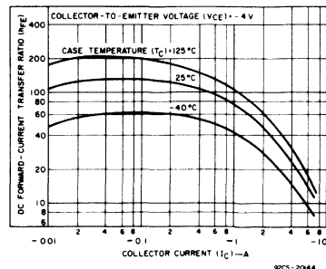
Fig. 3 - Typical dc beta characteristics for BD244-series types.
