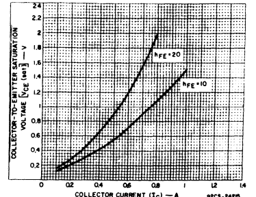
Fig. 6 - Typical saturation-voltage characteristics for RCP701, RCP703, RCP705, RCP707-series types.
