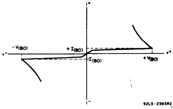
Fig.43 - Voltage-current characteristic for a diac.
