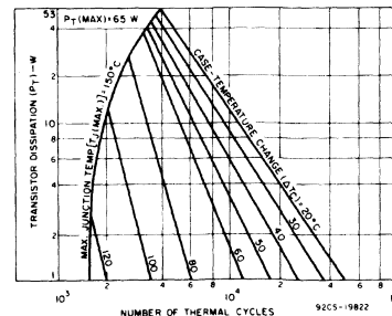
Fig. 3 - Thermal-cycling ratings for all types.
