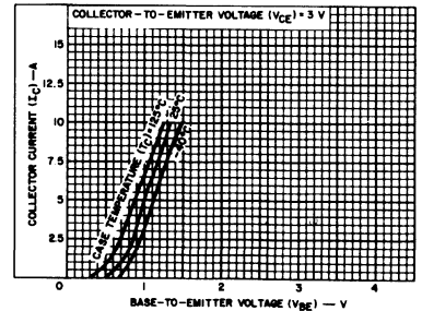
Fig. 7 - Typical transfer characteristics for all types.
