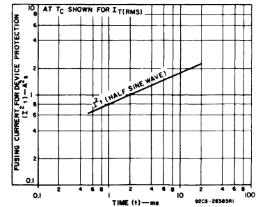
Fig. 7 - Fusing current as a function of time.
