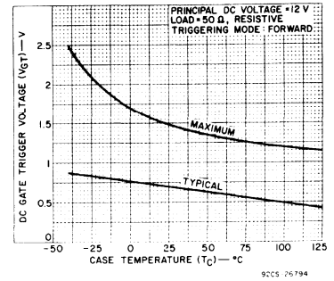
Fig. 15 — DC gate trigger voltage vs. case temperature for all types.
