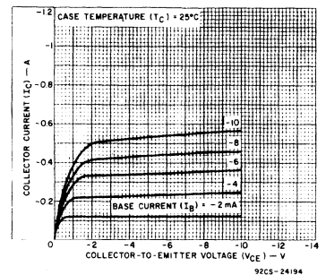
Fig. 9 - Typical output characteristics for RCP700, RCP702, RCP704, RCP706-series types.
