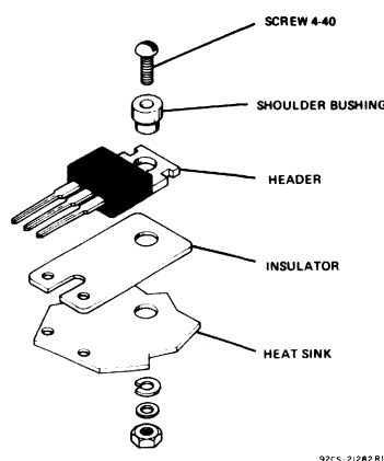
Fig. 8 - Mounting arrangements in which an isolating bushing is used to raise the head of the mounting screw above the plastic body of the VERSAWATT package.
