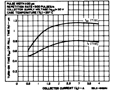
Fig. 13 - Typical saturated-time (turn-on or fall) as a function of collector current for both types.
