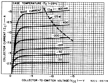
Fig. 14 - Typical output characteristics for 2N6246, 2N6247, and 2N6469.
