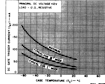
Fig. 13 - DC gate-trigger current (for I_{T1} and III^{+} triggering modes) vs. case temperature for T2800, T2802, T2850 series.
