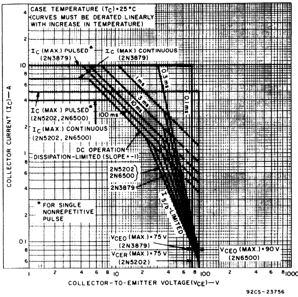
Fig. 5 - Maximum operating areas for 2N3879, 2N5202, and 2N6500.
