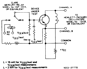
Fig. 6 - Basic configuration used to measure sustaining voltage V_{CE0}(sus) , V_{CE(sus)} , and V_{CEX}(sus) for n-p-n power transistors.
