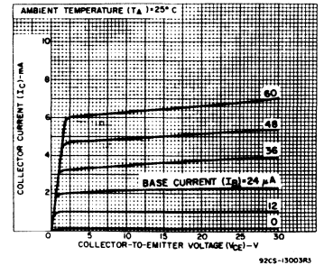
Fig. 8 – Typical output characteristics for 40407, 40408, and 40409.
