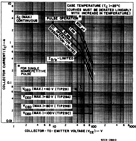
Fig. 1 — Maximum operating areas for TIP29-series.
