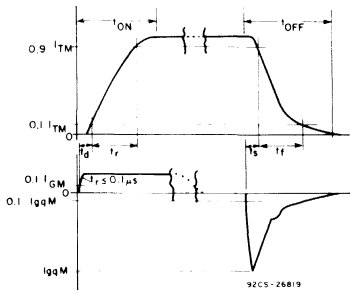
Fig. 37 — Relationship between anode current (on-state), gate-drive current, and time showing reference points for definition of t_{gt} ( t_{ON} ) and t_{gg} ( t_{OFF} ).
