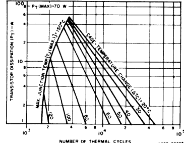
Fig. 1 - Thermal-cycling ratings.
