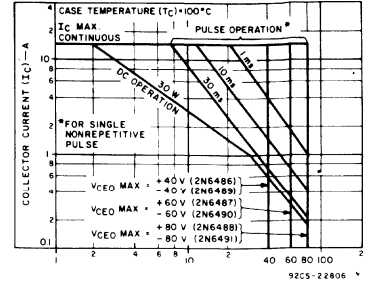
Fig. 5 - Maximum operating areas for all types.
