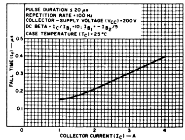
Fig. 7—Typical fall time vs. collector current.
