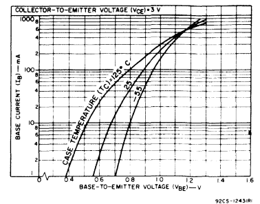
Fig. 6—Typical input characteristics.
