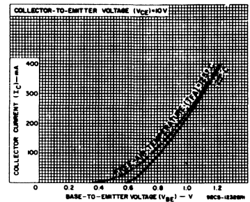
Fig. 8 - Typical transfer characteristics for 2N3053, 2N3053A, 40389, 40392.
