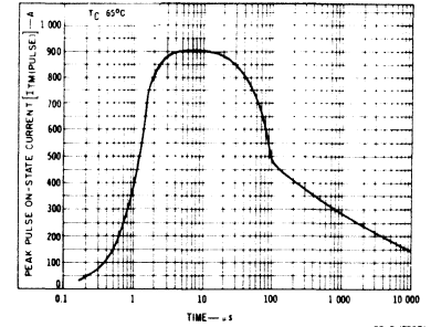
Fig. 1 — Peak pulse on-state current vs. time.
