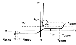
Fig. 1 — Principal voltage-current characteristic.
