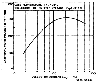
Fig. 5 — Typical gain-bandwidth product as a function of collector current.
