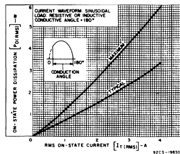
Fig. 1—Power dissipation vs. rms-on-state current for all series.
