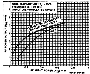
Fig. 2 - Typical output power as a function of input power at 27 MHz.
