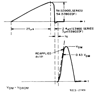
Fig. 40 — Oscilloscope display of trace switching ITR's (S3900 Series, S3902DF) showing circuit-commutated turn-off time ( t_q ).
