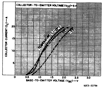
Fig. 13 - Typical transfer characteristics for 2N5038.
