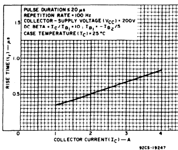
Fig. 8—Typical rise time vs. collector current.
