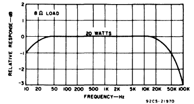
Fig. 6 - Typical frequency response.
