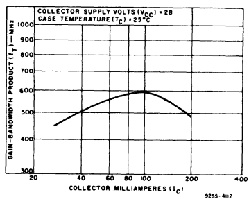
Fig. 8 - Gain-bandwidth product as a function of collector current for 2N3553.
