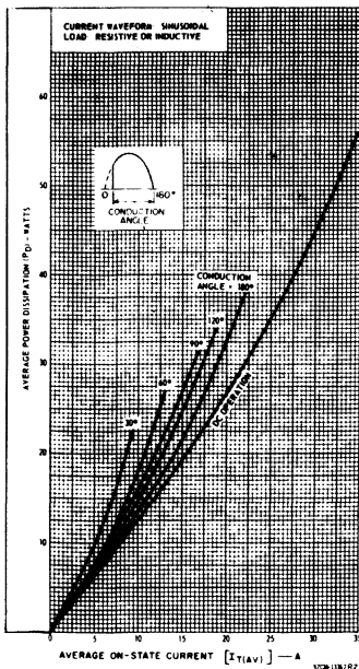
Fig. 1 — Power dissipation vs. on-state current.
