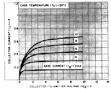
Fig. 14 - Typical output characteristics for RCP701, RCP703, RCP705, RCP707-series types.
