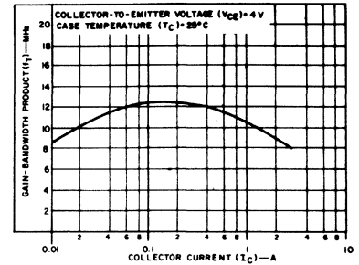
Fig. 5 - Typical gain-bandwidth product for all types. ♦
