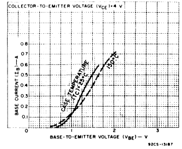
Fig. 6 – Typical input characteristics for 40411.
