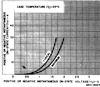
Fig. 6 - On-state current vs. on-state voltage for T2800, T2802, T2850 series.
