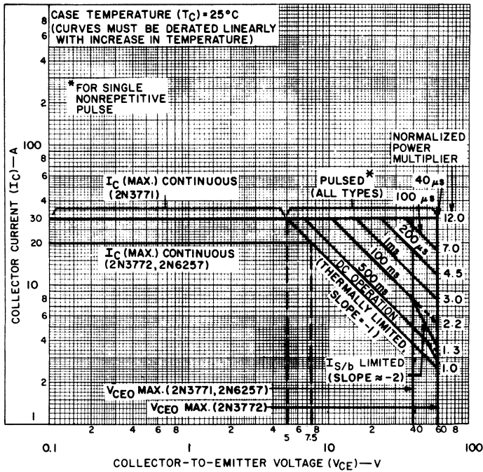
Fig. 7— Maximum operating areas for 2N3771, 2N3772, and 2N6257.
