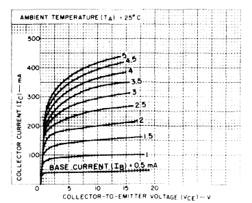
Fig. 21 - Typical high-current output characteristics for 2N1613, 2N2102, 41502.
