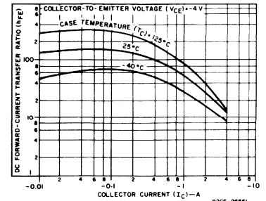
Fig. 6 - Typical dc beta characteristics for 2N6467 and 2N6468.
