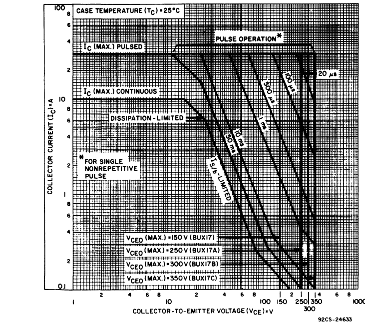
Fig. 1 - Maximum operating areas for all types.
