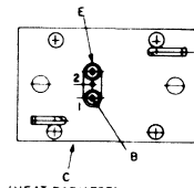
(HEAT RADIATOR) JEDEC TO-66 with Heat Radiator 40829, 40830, 40831
