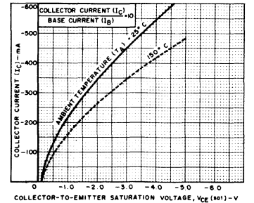
Fig. 6—Typical saturation-voltage characteristics for 2N4036.
