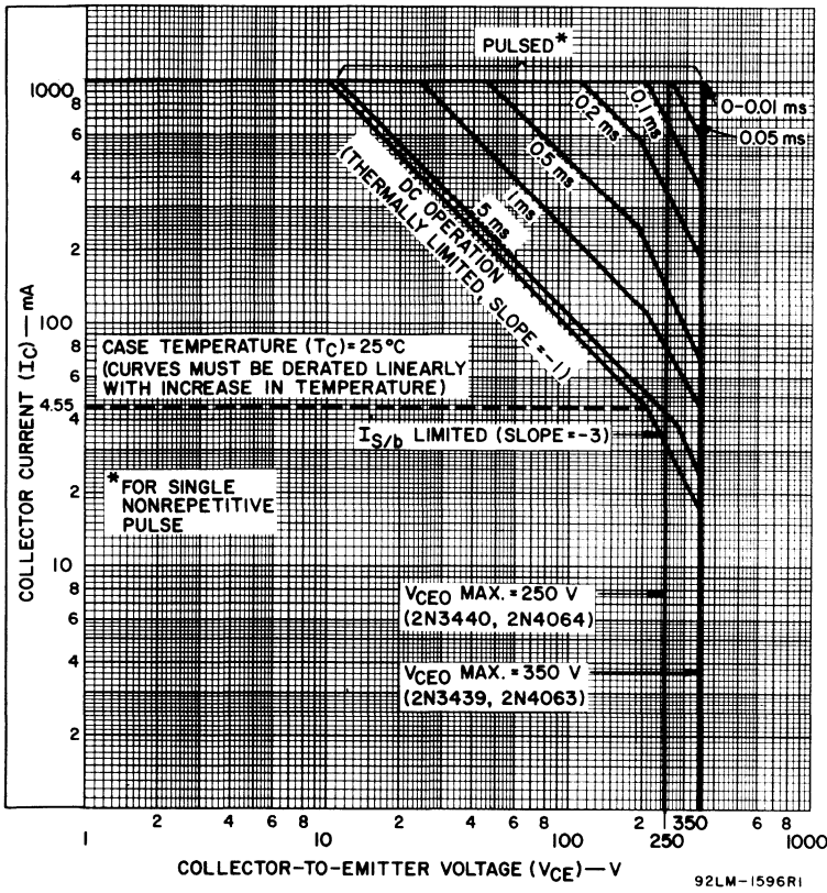
Fig. 4—Maximum operating areas for 2N3439, 2N3440, 2N4063 and 2N4064.
