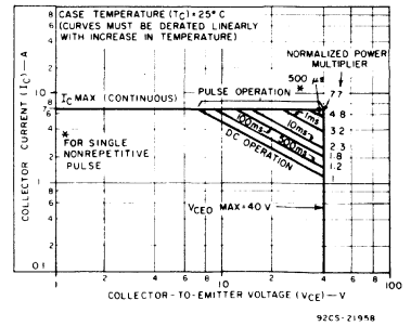
Fig. 3 - Maximum operating areas for RCA1C14.
