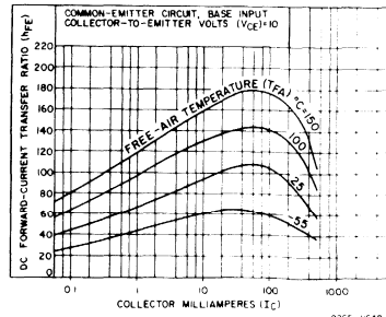
Fig. 3 - Typical dc beta characteristics for 2N1893, 2N2405.
