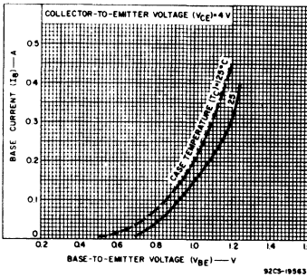
Fig. 21 - Typical input characteristics for 2N6262.
