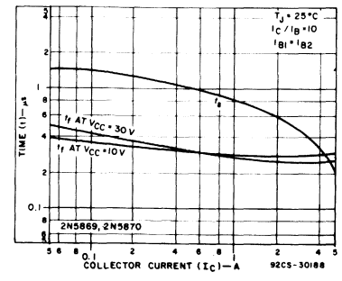
Fig. 6 - Turn-off-time characteristics.
