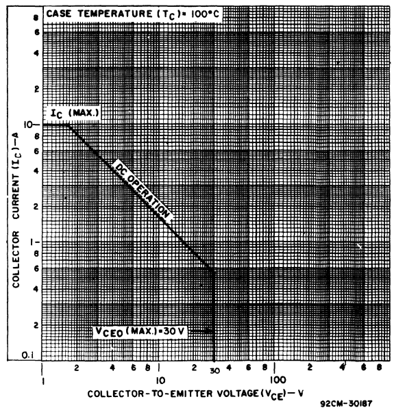
Fig. 3 - Maximum operating areas at T_C = 100^\circ\text{C} .
