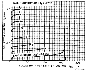
Fig. 20—Typical output characteristics for 2N6264 and 40913.
