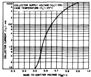
Fig. 3 - Typical transfer characteristic.
