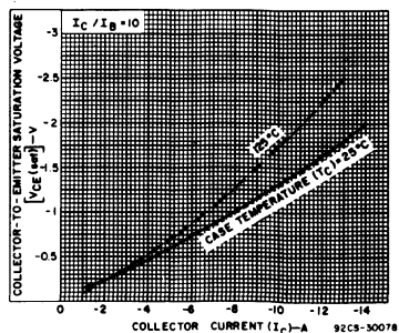
Fig. 10 – Typical saturation voltage characteristics for MJ15002.
